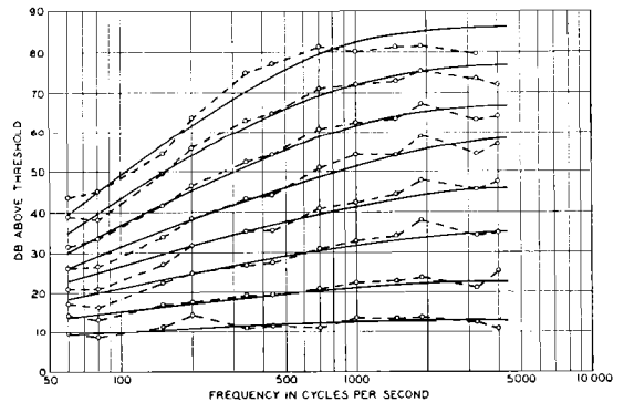
FIG. 21. Loudness levels of pure tones—A comparison with Kingsbury's data.
