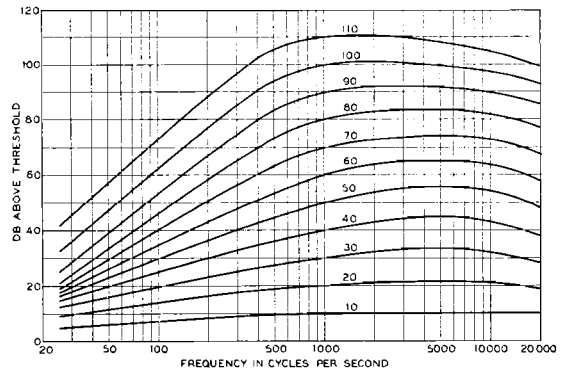
FIG. 3. Loudness level contours.
